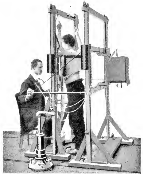
FIG. 75.—Wenckebach screening stand. (Siemens.)
